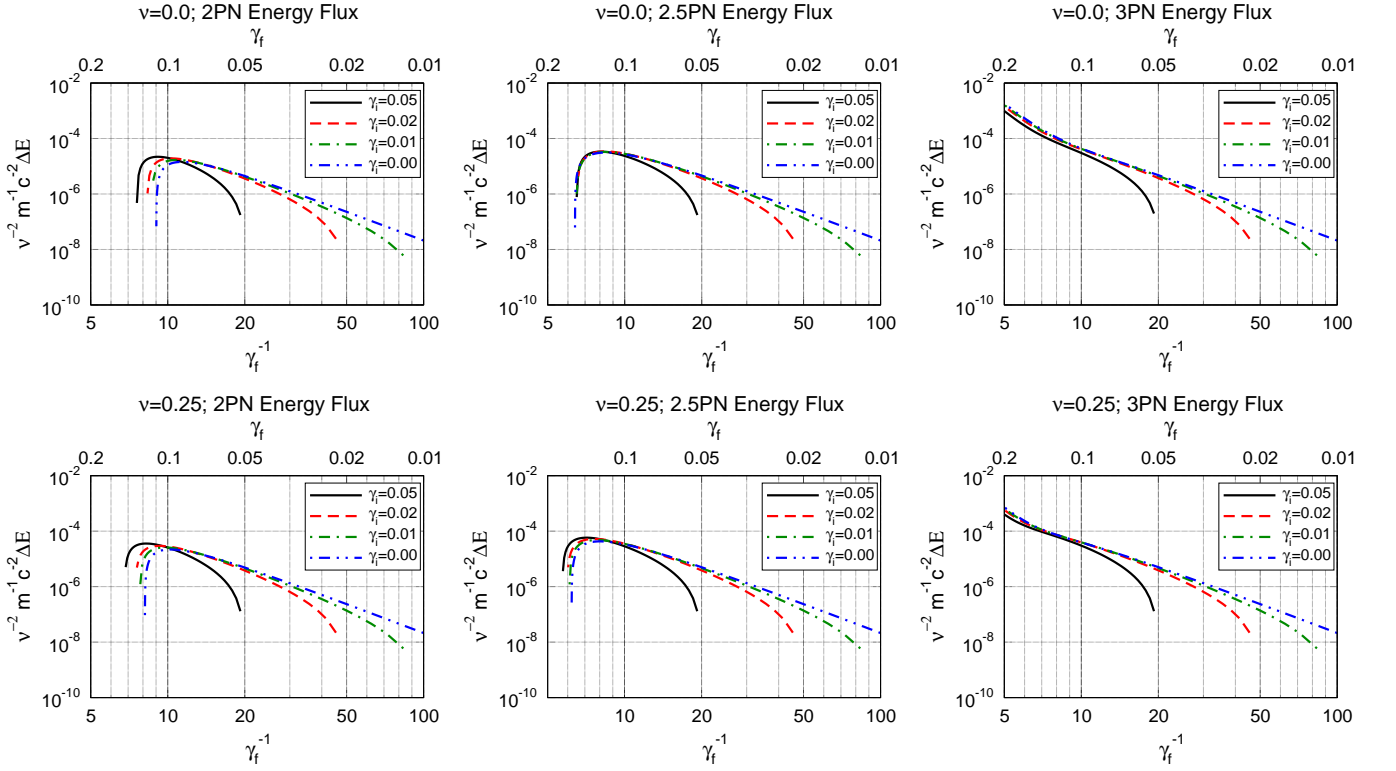
FIG. 2: Similar to Fig. 1 but for total energy radiated in units of v^2 c^2 m , during the head-on infall of two compact objects from a initial separation z_i in ADM coordinates (related to the parameter \gamma_i ) to a final separation of z_f (corresponding parameter \gamma_f = Gm/c^2 z_f ).
