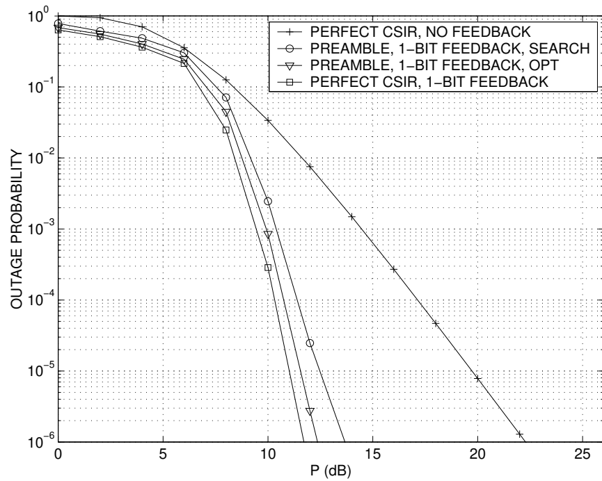
Fig. 7. Comparison of the two upper bounds obtained by (i) quantizer search and (ii) analytical optimization – outage probability versus power constraint for M = 4 transmit antennas, frame length T = 1000 , rate R = 2 bits/s/Hz.
