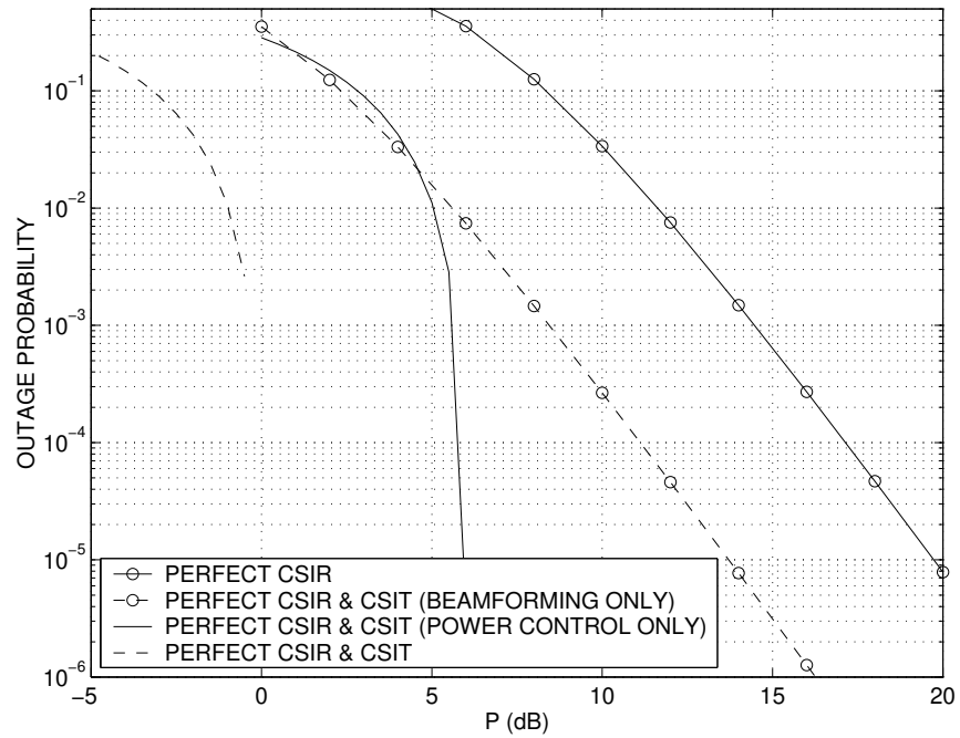
Fig. 2. Performance gains from feedback – outage probability versus average power constraint for rate R = 2 bits/s/Hz, M = 4 transmit antennas, frame length T = 1000 . For the Perfect CSIR & CSIT curve, outage is zero for P larger than the plotted range.
