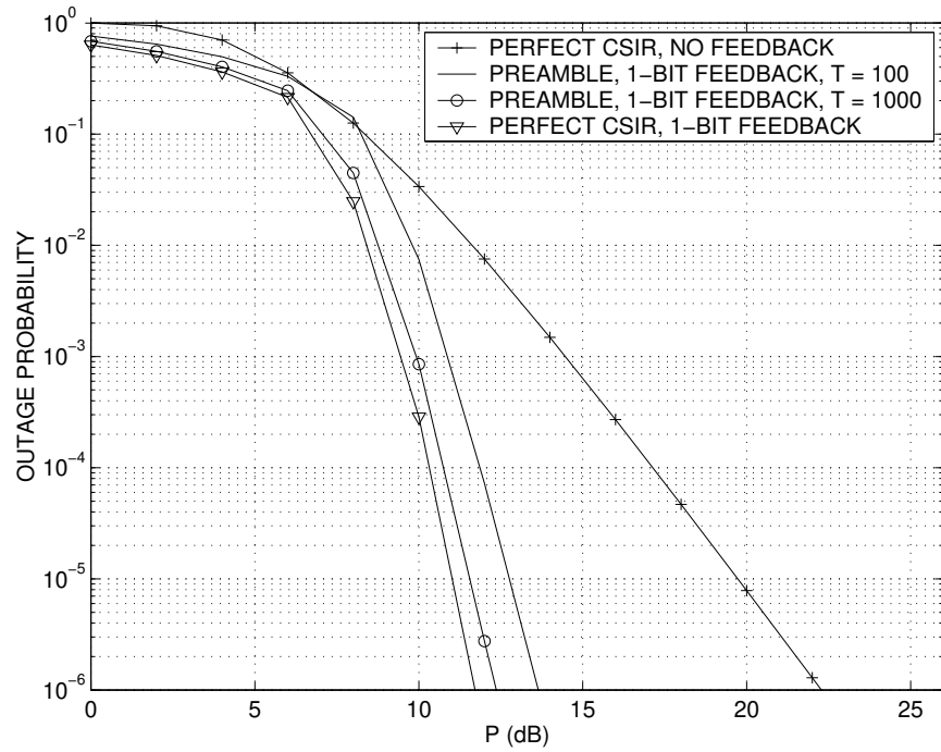
Fig. 6. Effect of frame length ( T ) on outage probability – outage probability versus power constraint for M = 4 transmit antennas, rate R = 2 bits/s/Hz.
