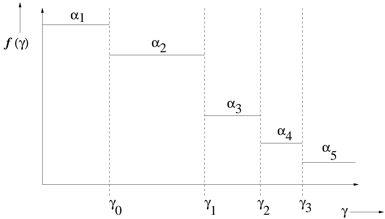
Fig. 1. Power control function
