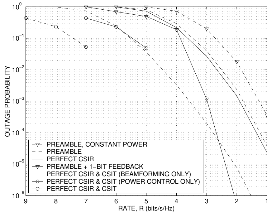
Fig. 3. Outage probability versus transmission rate for M = 4 transmit antennas, average power constraint P = 14 dB, frame length T = 1000 . For the Perfect CSIR & CSIT and the Perfect CSIR & CSIT (Power control only) curves, outage is zero for R smaller than the plotted range.
