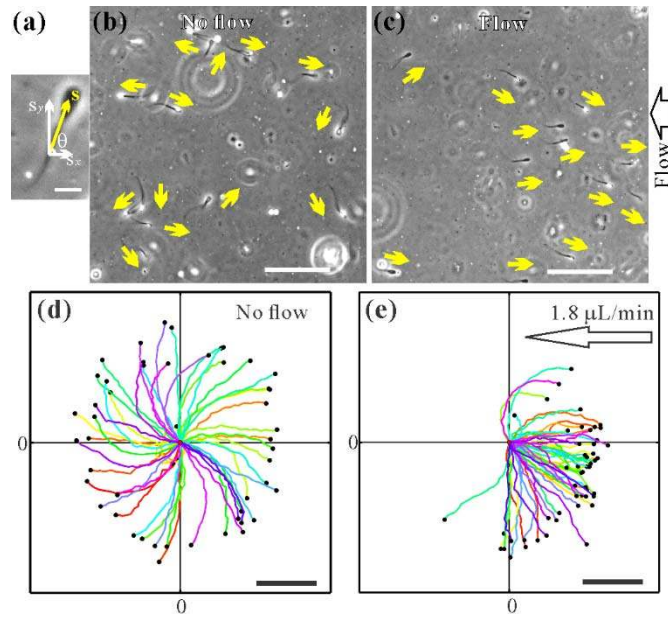
FIG. 2 Emergence of upstream swimming and CW swimming chirality. (a) Sperm head orientation is represented by the unit vector, s , where \theta is the angle with respect to x -axis. Scale bar: 15 \mu\text{m} . (b) and (c) Micrograph (422.5 x 422.5 \mu\text{m} ) of sperm swimming in the absence/presence of the flow (4.5 \mu\text{L}/\text{min} ). Yellow arrows denote the sperm head orientation. Scale bar: 100 \mu\text{m} . (d) and (e) Trajectories of \sim 50 sperm, each is sampled at 8.91 Hz and 2.81 s long, when there is no flow (d), and when a critical flow rate is exceeded (e). Clockwise (CW) chirality (with an exception of \sim 6\% of the sperm) is demonstrated in (d). Emergence of directional swimming pattern is clearly shown in (c) and (e). Flows are applied in the -x direction. Scale bar: 100 \mu\text{m} .
