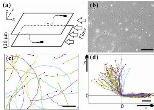
FIG. 1 Sperm structure, trajectory chirality, and near-surface swimming. (a) Schematic of experimental setup. Each bull sperm has a paddle-shape head, with approximate dimensions of 10\ \mu\text{m} long, 5\ \mu\text{m} wide, and roughly 1\ \mu\text{m} thick. The head is directly connected to a single flagellum that is about 50 - 60\ \mu\text{m} long and tapers from 1\ \mu\text{m} in diameter at the connection to 200\ \text{nm} at the tail end. Mean swimming speed is close to 120\ \mu\text{m/s} . Sperm travelling along the surfaces of a microfluidic channel with 2.47\ \text{mm} width and 120\ \mu\text{m} height. Fluid flow is applied in -x direction. (b) A micrograph ( 570 \times 426\ \mu\text{m} ) of sperm swimming along the lower surface of the central portion of the microfluidic channel. Scale bar: 100\ \mu\text{m} . (c) Trajectories (1-6.30s long) of sperm in the absence of the flow. Each colored line is a sperm track that ends at the black dot. CW chirality is seen in the trajectories. Scale bar: 100\ \mu\text{m} . (d) Trajectories (1.78 s long) of 30 sperm swimming toward the side wall of the microfluidic channel, and the coordinate (0,0) marks the point where the sperm hits the side wall. The sperm continue to move along the sidewall (or x -axis). Red/black dots are starting/ending positions of the tracks. Scale bar: 25\ \mu\text{m} .
