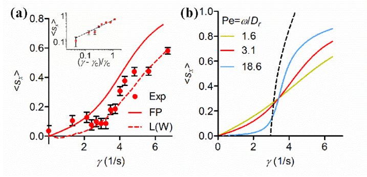
FIG. 4 Onset of upstream swimming via a saddle-node transition. (a) The average value of sperm head orientation unit vector along the x -direction (or against the flow direction) \langle s_x \rangle versus shear rate \gamma . Red dots are experimental measurements, red solid line is the solution of the Fokker-Planck equation, and dashed line is the results of Langevin simulation taking into account the wiggling motion. Error bars show standard errors of the mean. Inset: a power law with exponent of 0.53 \pm 0.05 is observed above \gamma_c for measured \langle s_x \rangle versus \gamma curve. The black dashed line is a guideline with an exponent of 0.5. (b) Numerical solution of the Fokker-Planck equation showing that the transition curve becomes steeper with increasing Péclet number (Pe). In the high Pe asymptotic limit, it approaches the black dashed line described by
