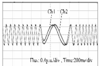
Fig.28.Fluxes during speed reversal Ch1: \Psi_{\alpha 1} Ch2: \Psi_{\beta 1}
