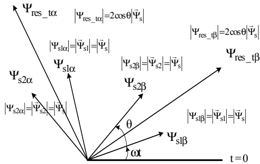
Fig.12. Description of different phasors
