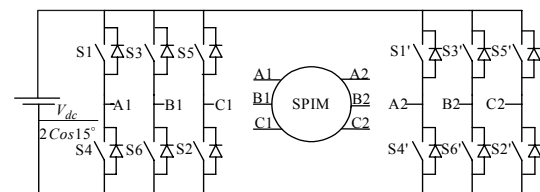
Fig.2. SPIM Drive
