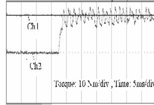
Fig.21.Ch1: m_d^* Ch2: m_d
