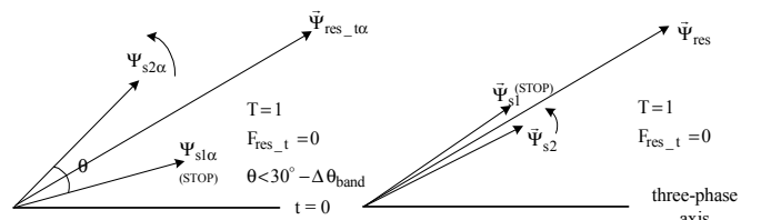
Fig.17.a. Time phasor
