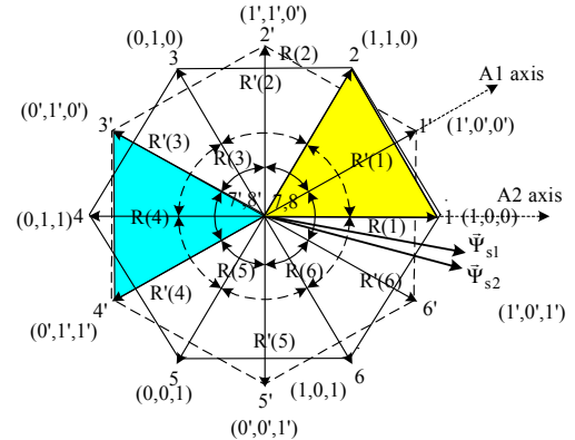
Fig.13. Sector identification
