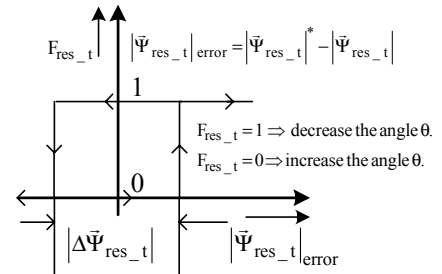
Fig.14. Angle Controller
