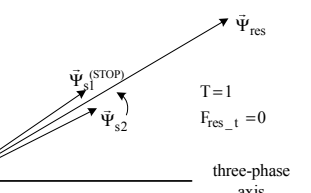
Fig.17.b.Space phasor
