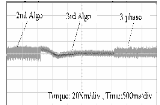
Fig.38. Torque transients at no load
