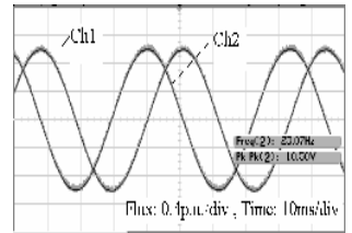
Fig.36.Ch1 : \Psi_{res\beta} Ch2 : \Psi_{res\alpha}
