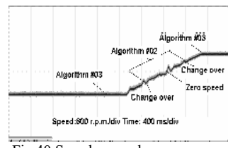
Fig.40. Speed reversal : -350 < \omega < 350 : Algorithm#02 \omega < -350 & \omega > 350 : Algorithm#03
