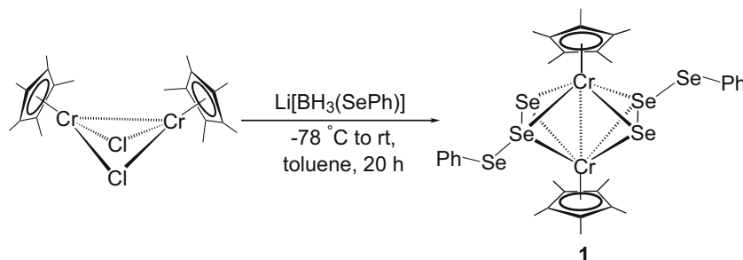
Scheme 1. Synthesis of 1.
