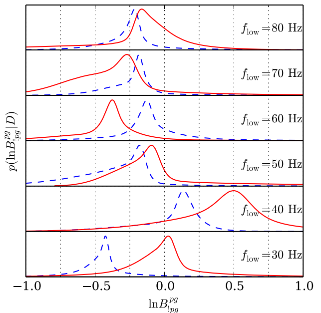
FIG. 1. Distributions of \ln B_{1pg}^{pg} due to sampling uncertainty when analyzing GW170817 data with different values of f_{\text{low}} . The solid red curves assume high-spin priors ( |\chi_i| \leq 0.89 ) and the dashed blue curves assume low-spin priors ( |\chi_i| \leq 0.05 ).
